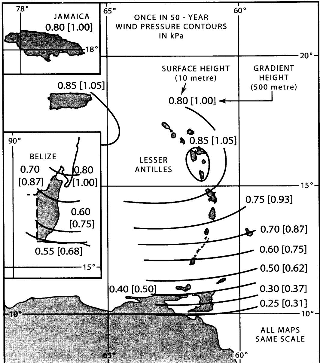
Figure 1 - Regional Map of Wind-pressure Contours (from CUBiC)
