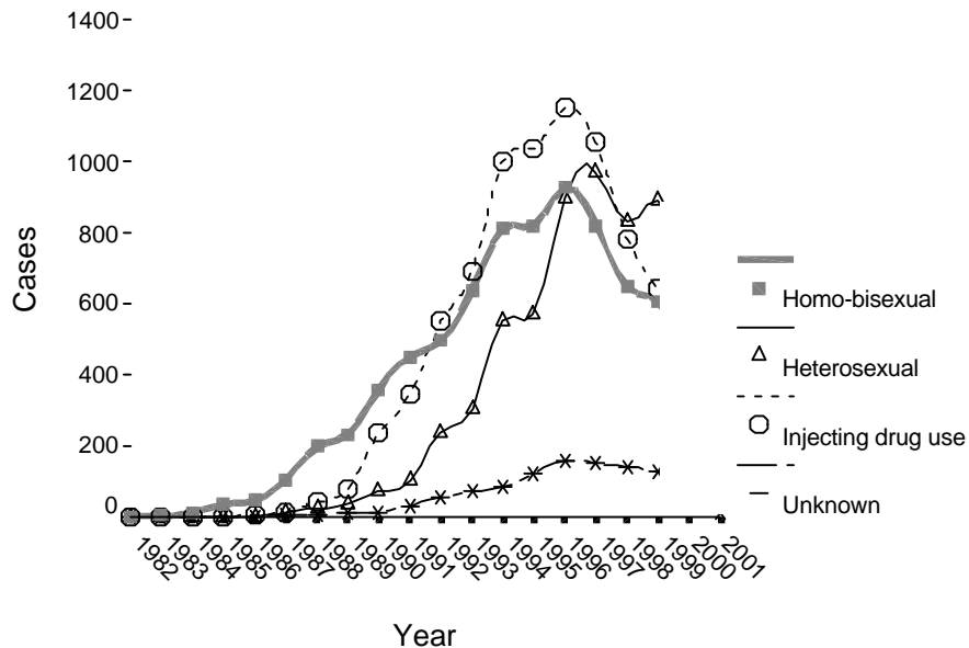
Number of AIDS cases by year of diagnosis and exposure category, Southern Cone, 1982-1999
