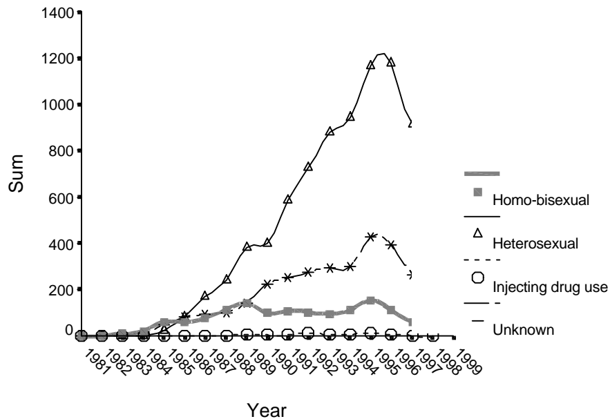
Number of AIDS cases by year of diagnosis and exposure category, Caribbean, 1981-1997
