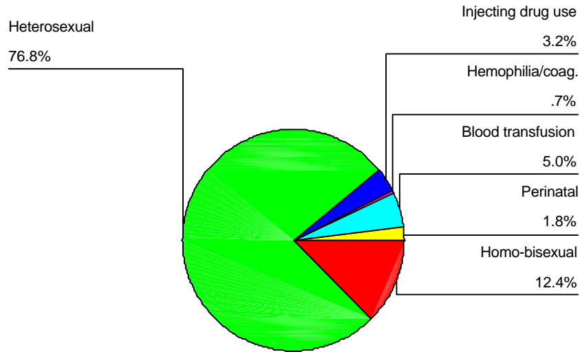
Percent distribution of total cumulative AIDS cases by a known exposure category, Latin Caribbean, 1981-Dec. 2001
