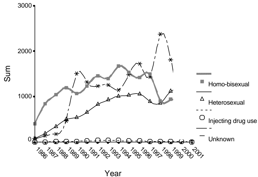
Number of AIDS cases by year of diagnosis and exposure category, Mexico, 1986-1999
