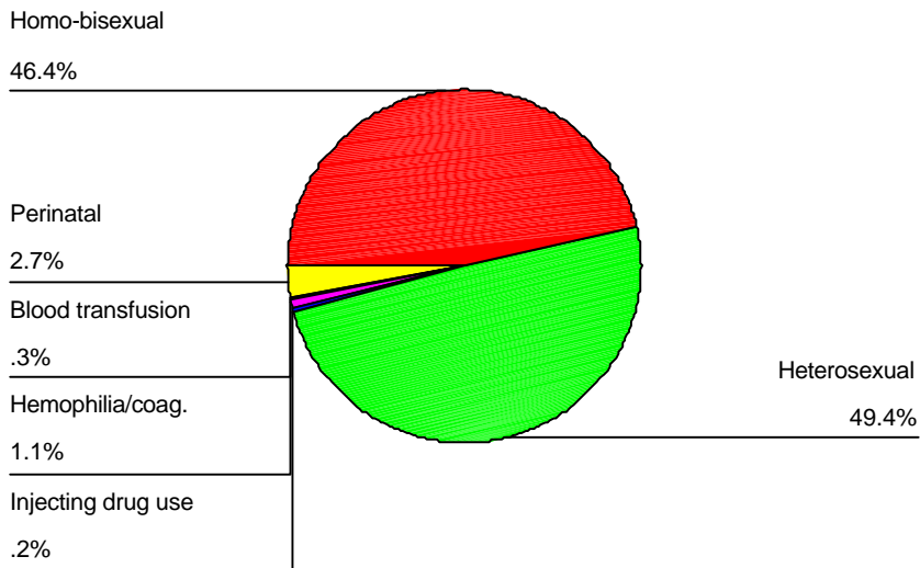
Percent distribution of total cumulative AIDS cases by a known exposure category, Andean Area, 1983-Dec. 2001
