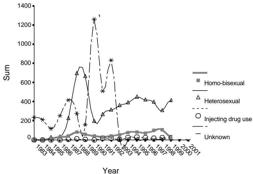
Number of AIDS cases by year of diagnosis and exposure category, Latin Caribbean, 1983-1999
