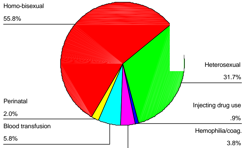
Percent distribution of total cumulative AIDS cases by a known exposure category, Mexico, 1983-Dec. 2001
